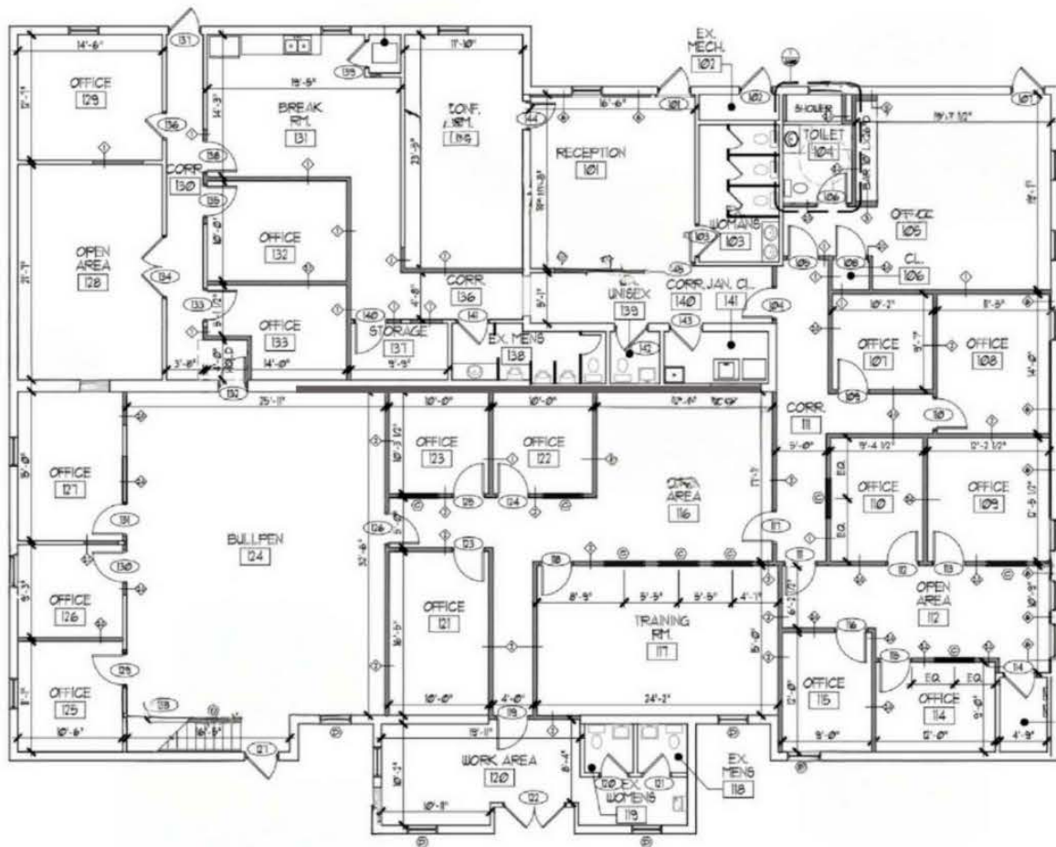
1 FIRST FLOOR PLAN SCALE: 1/8" = 1'-0"
