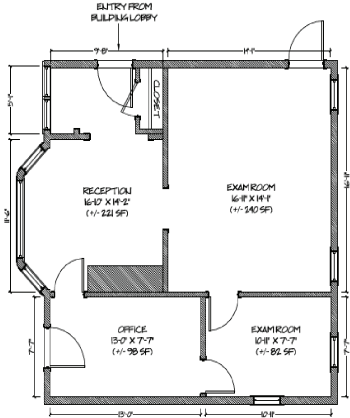
Floor Plan Not Drawn to Scale
