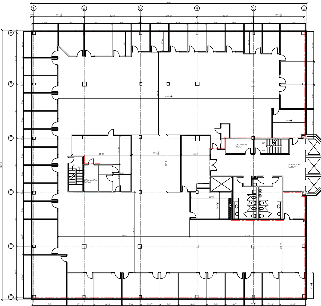
① 5TH FLOOR PLAN SCALE: 1/8" = 1'-0"
